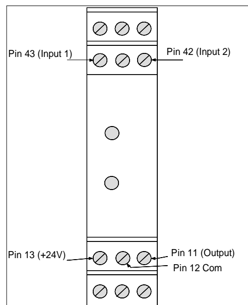
Figure 1: Wiring Diagram for ATE-30
