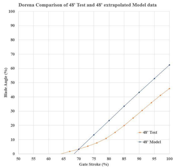
Figure 5 48' Model and Test blade to gate
