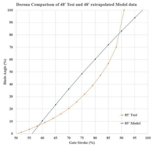
Figure 7 85' Model and Test blade to gate
