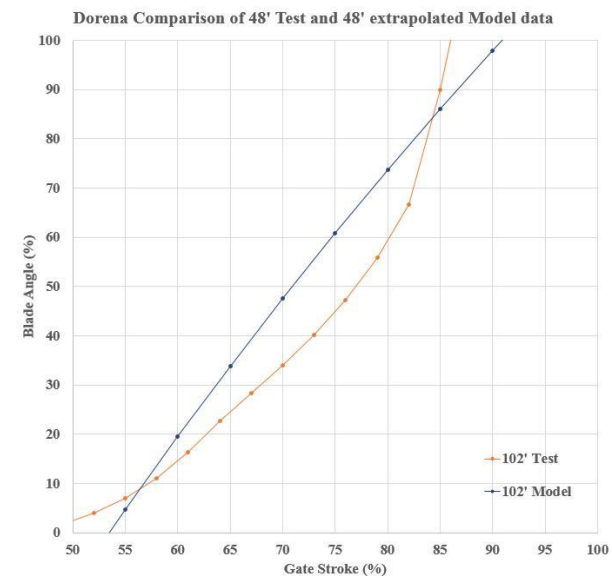
Figure 8 102' Model and Test blade to gate
