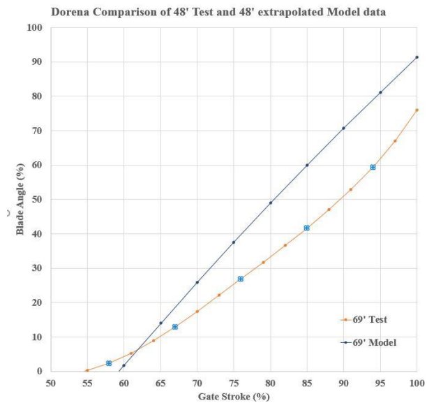
Figure 6 68' Model and Test blade to gate
